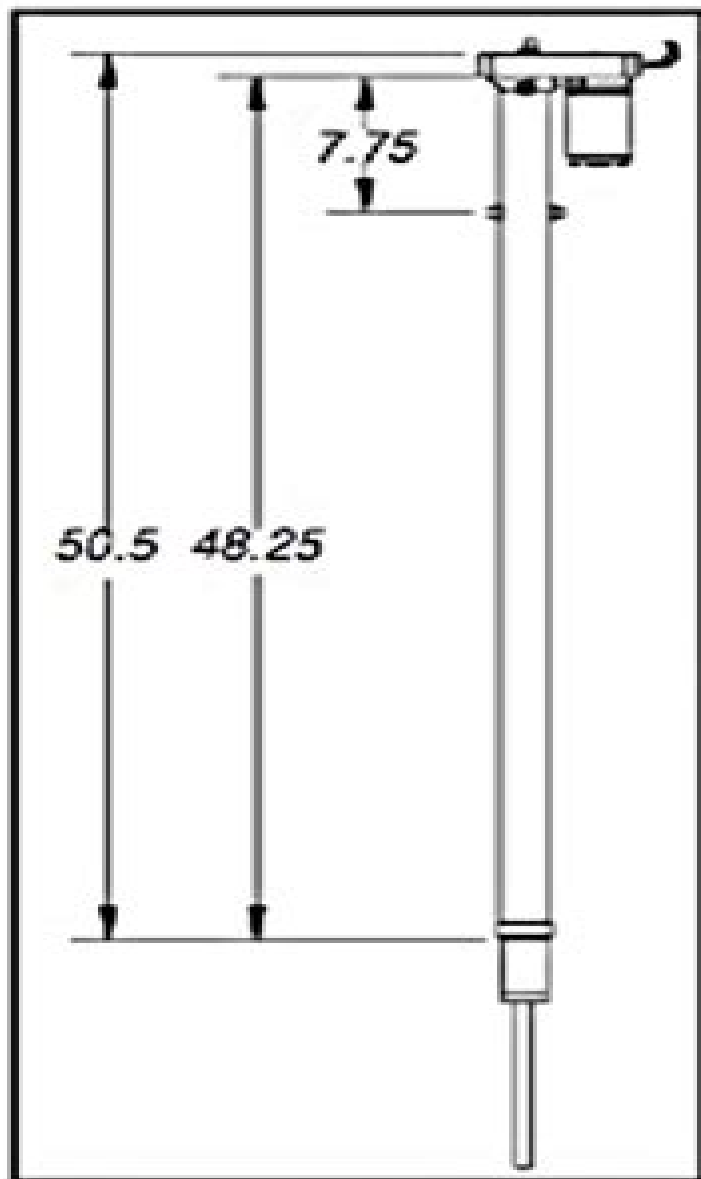
40° Venture Actuator with 18:1 High Speed Motor #014-168956
