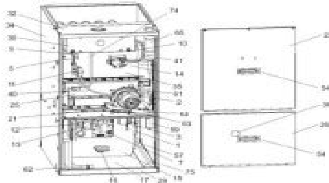
Figure 1: UPRFLOW NATURAL GAS FURNACES (82%)
