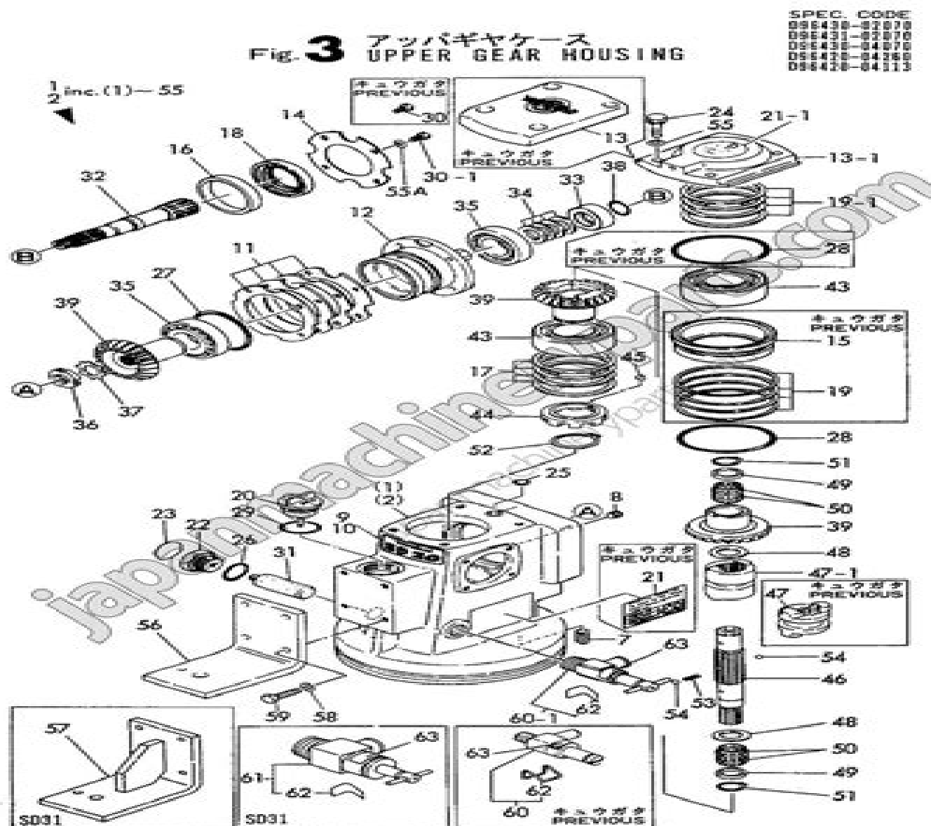
Fig.3.UPPER GEAR HOUSING
