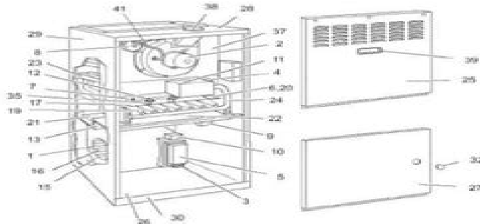
Figure 1: MULTI-POSITION NATURAL GAS FURNACES (80%)
