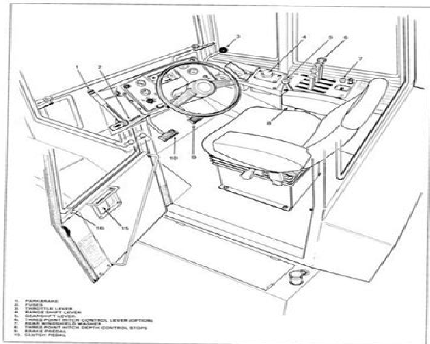
Cab Controls and Instruments
