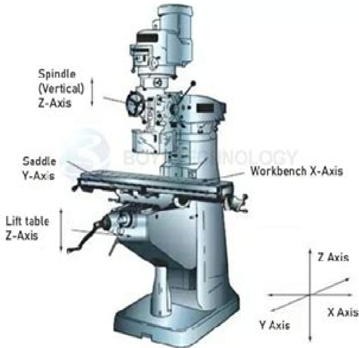
XYZ Direction Movement of Vertical Milling Machine
