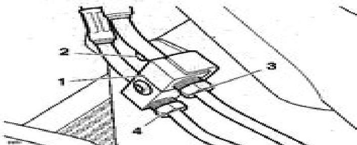
1. Front brake hose connector housing 2. Fixing 3. Front brake line from master cylinder 4. Front brake line to calipers
