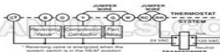
Figure 7. Typical wiring diagram for heat pump with reversing valve energized in HEAT
