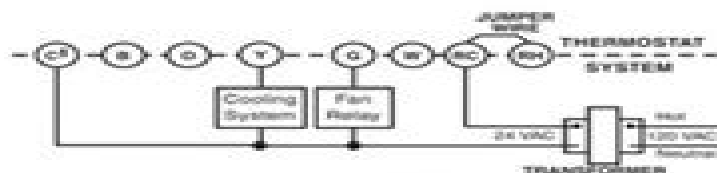
Figure 3. Typical wiring diagram for cool only, 3-wire, single transformer systems
