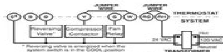
Figure 6. Typical wiring diagram for heat pump with reversing valve energized in COOL
