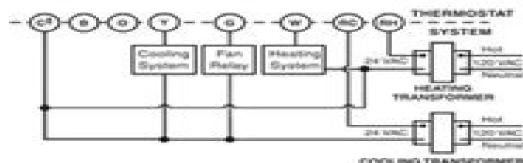
Figure 5. Typical wiring diagram for heat/cool, 5-wire, two-transformer systems
