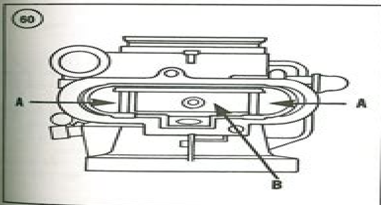
FLOAT LEVEL ADJUSTMENT (1994-1996 MODELS)
