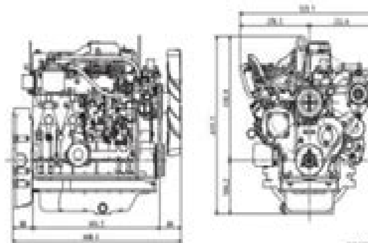
4TNV84-Z
