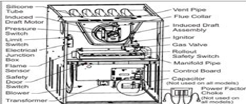
FIGURE 1: Component Location - 80% Single & Two Stage Models
