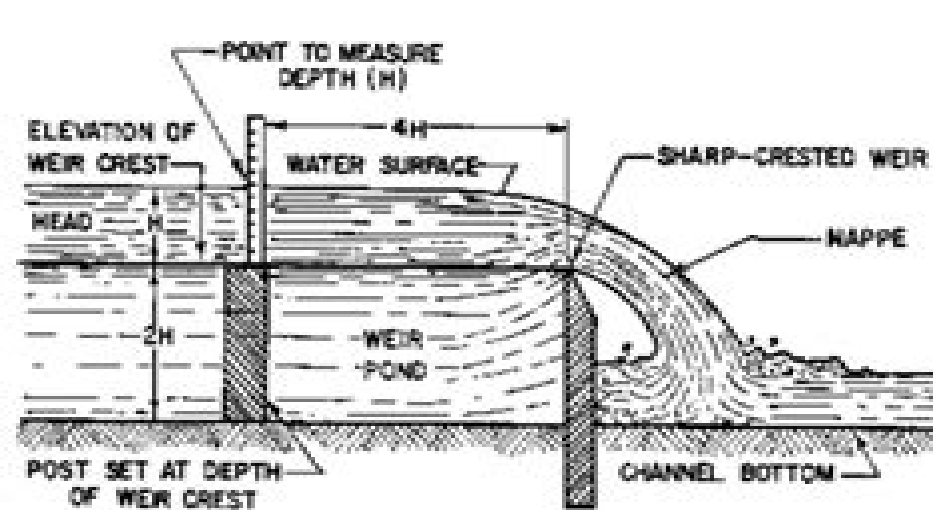
Common Types of Sharp Crested Weirs
