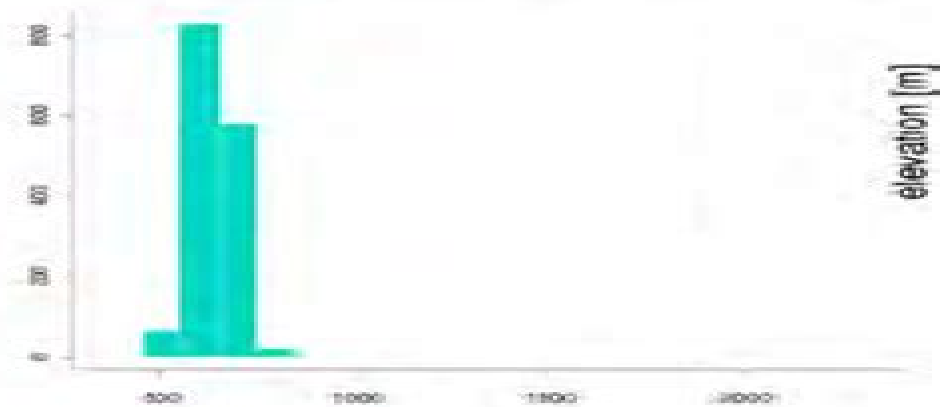
Ecoregion 55 (Bavarian Hills and Gravel Plains)
