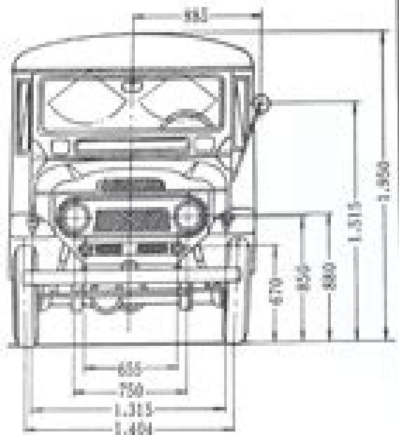
FIAT-V MAJOR DIMENSIONS ( mm )
