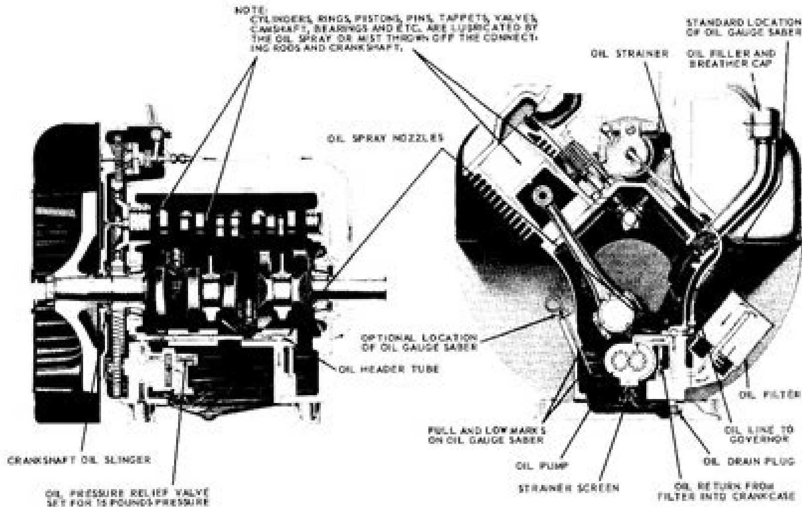
Fig. 3 LUBRICATION SYSTEM
