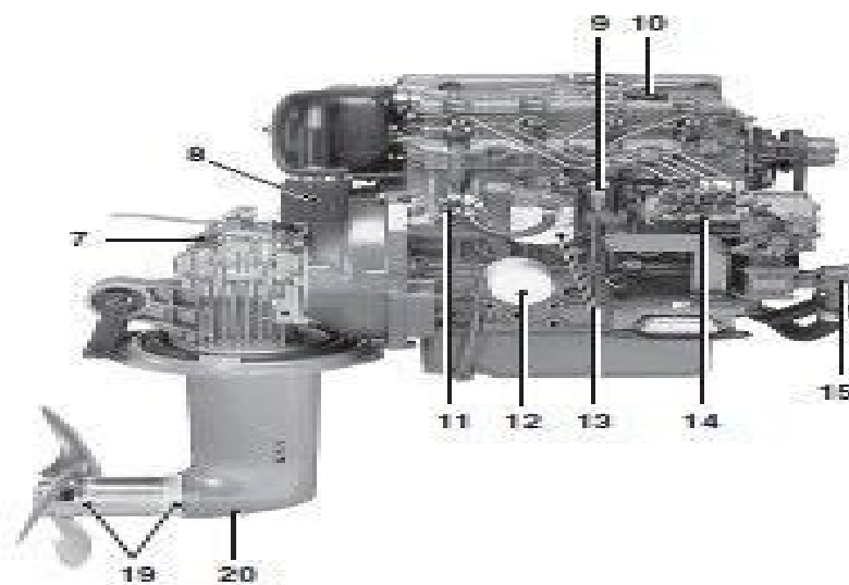
D2-55 A/B with sail-drive MS25S
