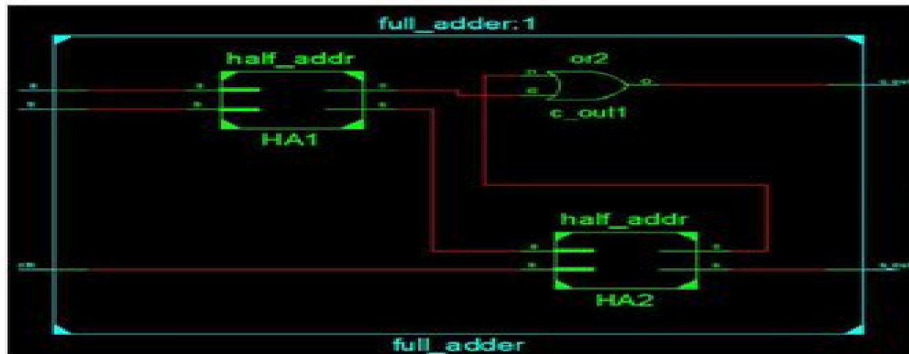
Figure 4.13 RTL Schematic for Full adder using half adders
