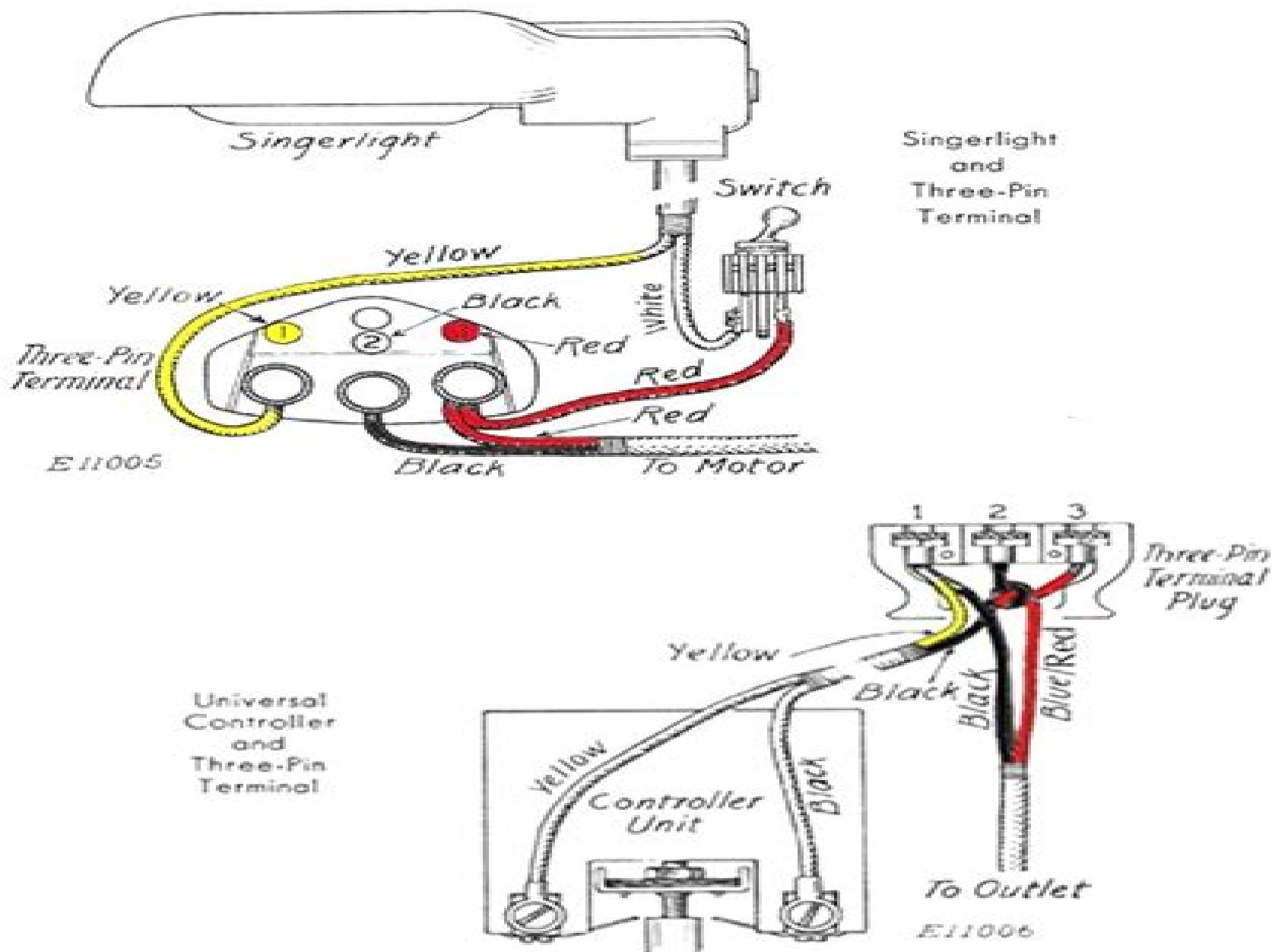
Wiring Diagrams of Connections to Series 3 and Series CA6 Motors, used with Singer 221-1 Machine.
