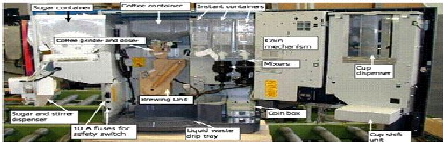
BRIO 250: VIEW WITH DOOR OPEN
