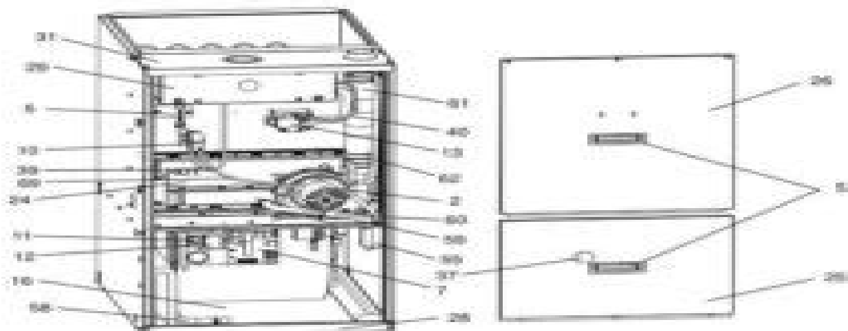
Figure 1: CONDENSING-UPFLOW NATURAL GAS FURNACES
