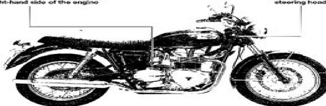
The engine number is stamped into the top of the crankcase on the right-hand side of the engine
