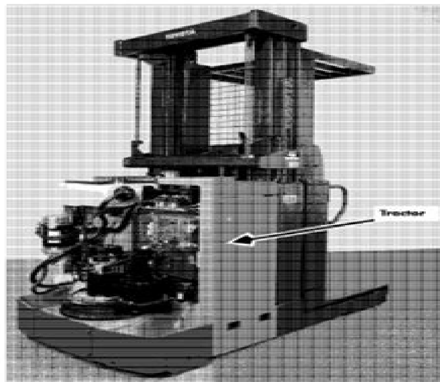
Figure 3-2. Model 7BPUE15, Tractor View, Cover Removed
