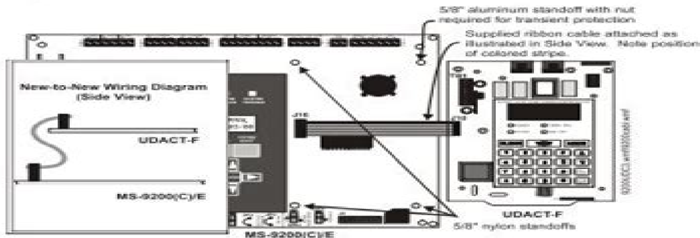
Figure 1: New-to-New Internal UDACT-F Installation (Top View and Side View)
