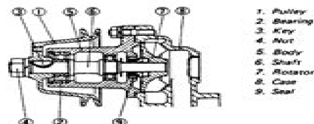
Fig. 39. Water Pump
