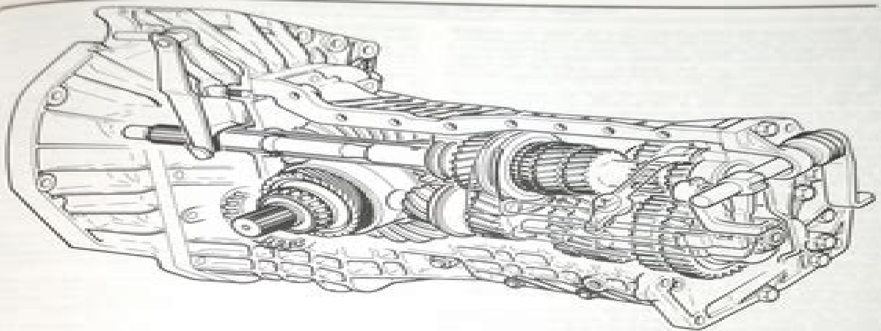
Fig. 6.1 Gearbox and differential unit — type 367 (4-speed) (Sec. 1)
