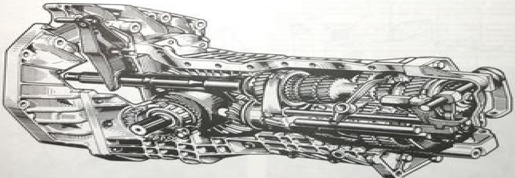
Fig. 6.2 Gearbox and differential unit — type 369 (5-speed) (Sec. 1)
