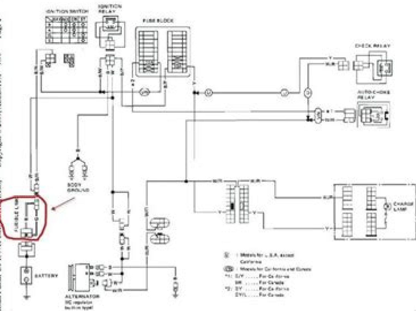
Fig. 2.39 Charging System Wiring Circuit
