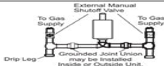
FIGURE 8: Gas Piping
