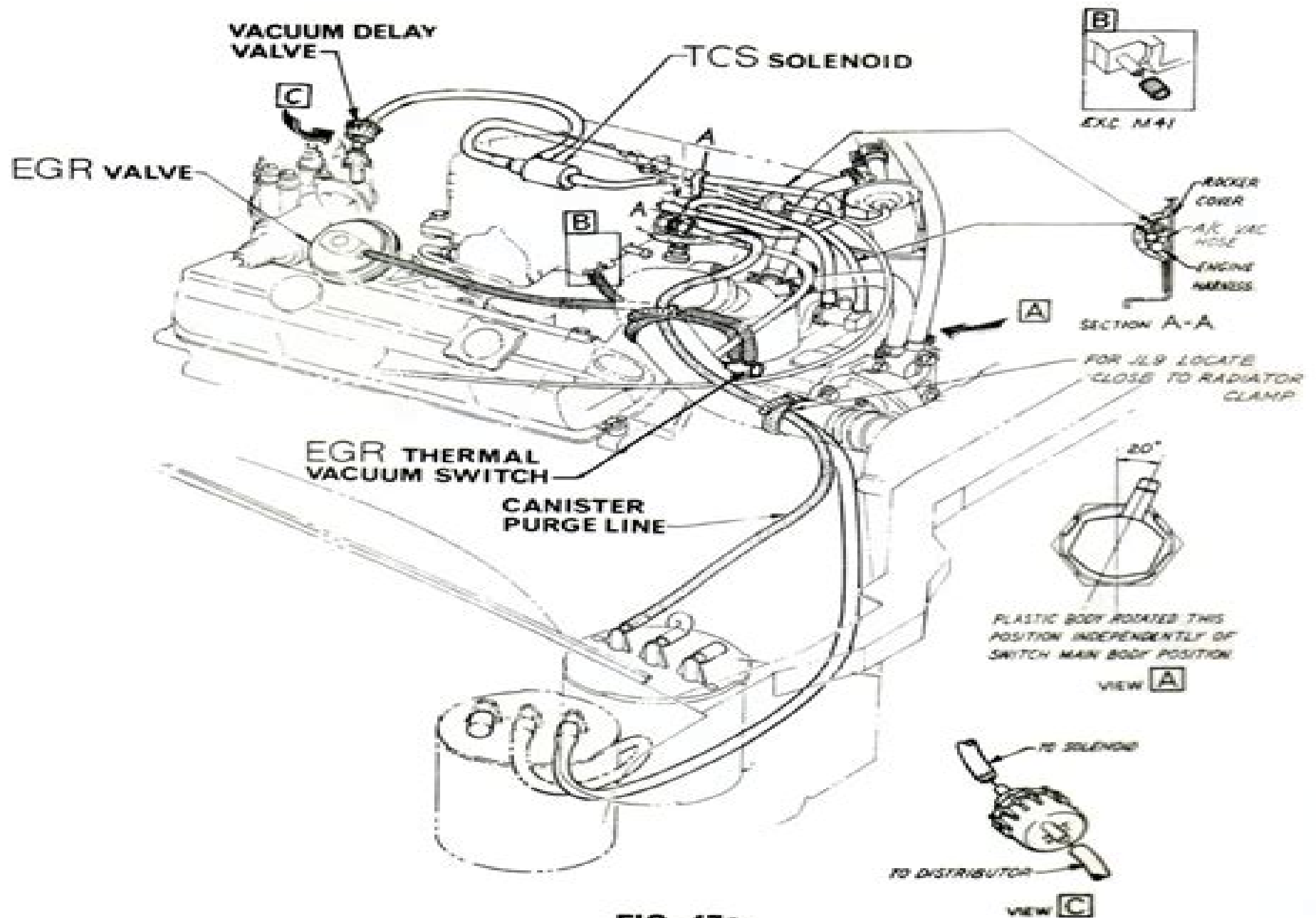
FIG. 47a 5.0 LTR EMISSION HOSE CONNECTIONS
