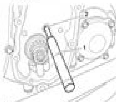
1. Camshaft Timing Pin (T480040) 2. Timing hole in position
