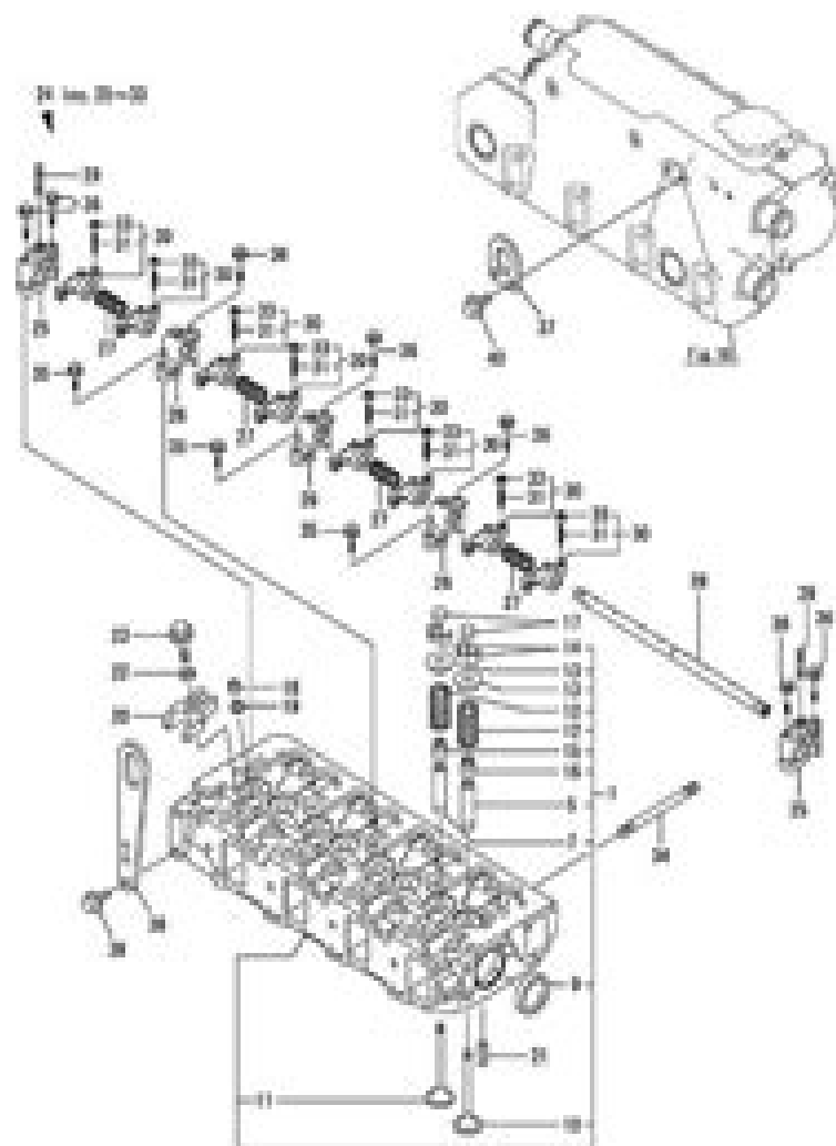
Fig.7. CYLINDER HEAD
