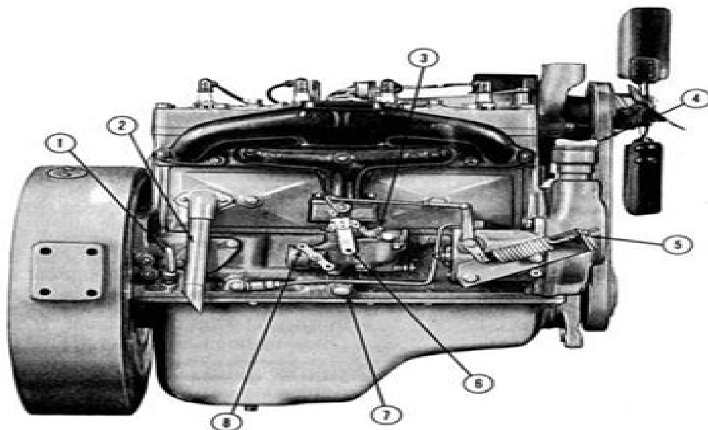
RIGHT SIDE — WAUKESHA MODEL FC
