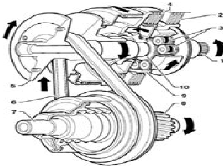
Fig. 21: Pulleys & gear train
