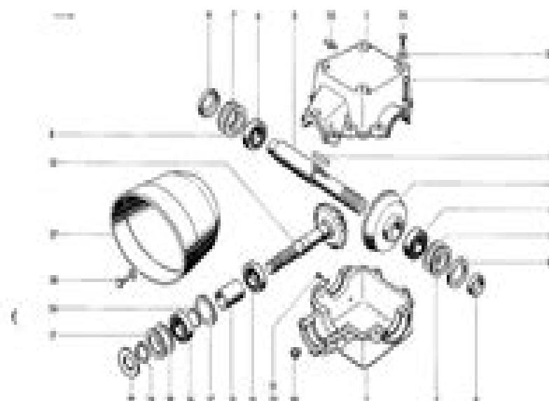
Exploded view
