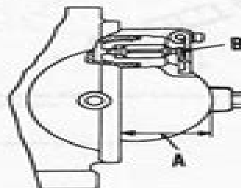
Fig. HN13-4—Float height (A) should be 21 MM with tang (B) just touching inlet needle.
