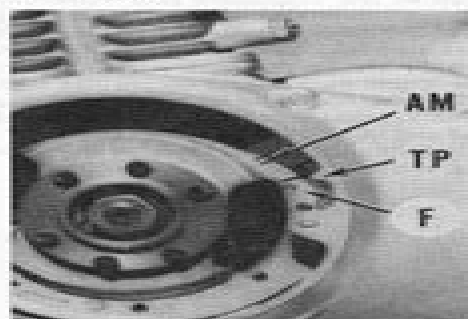
Fig. HN13-1—View of flywheel timing marks and timing pointer (TP) on crankcase cover.
