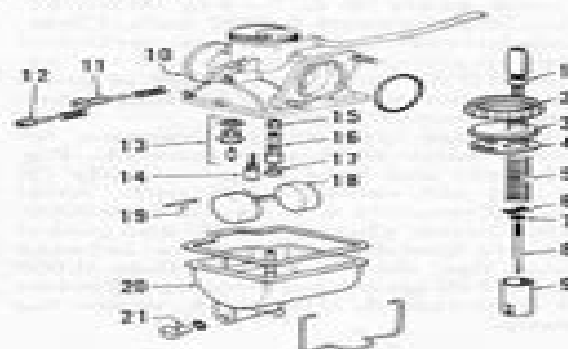
Fig. HN 12-3—Exploded view of carburetor used on XR75.
