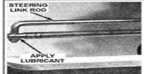
Fig. 13 Apply Yamaha All Purpose Grease to the steering link rod joint
