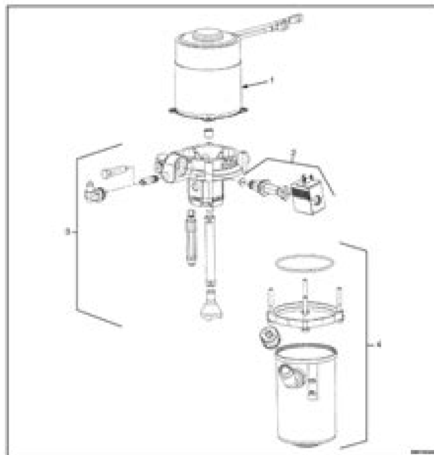
Figure 8. Hydraulic Unit (A24S)
