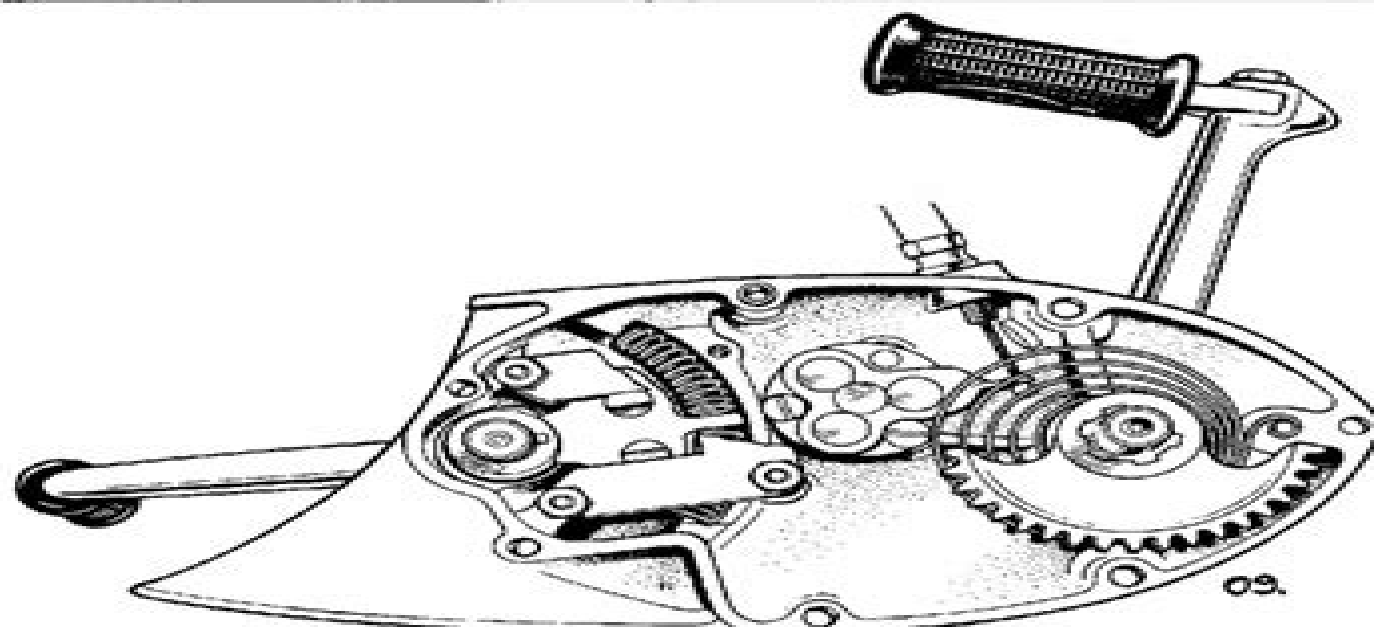
Fig. D3. Gearbox outer cover, showing gearchange mechanism, clutch operating mechanism and kick-start quadrant
