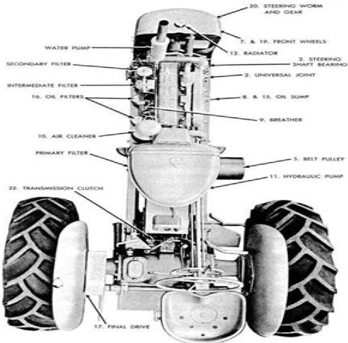
LUBRICATION AND SERVICE CHART
