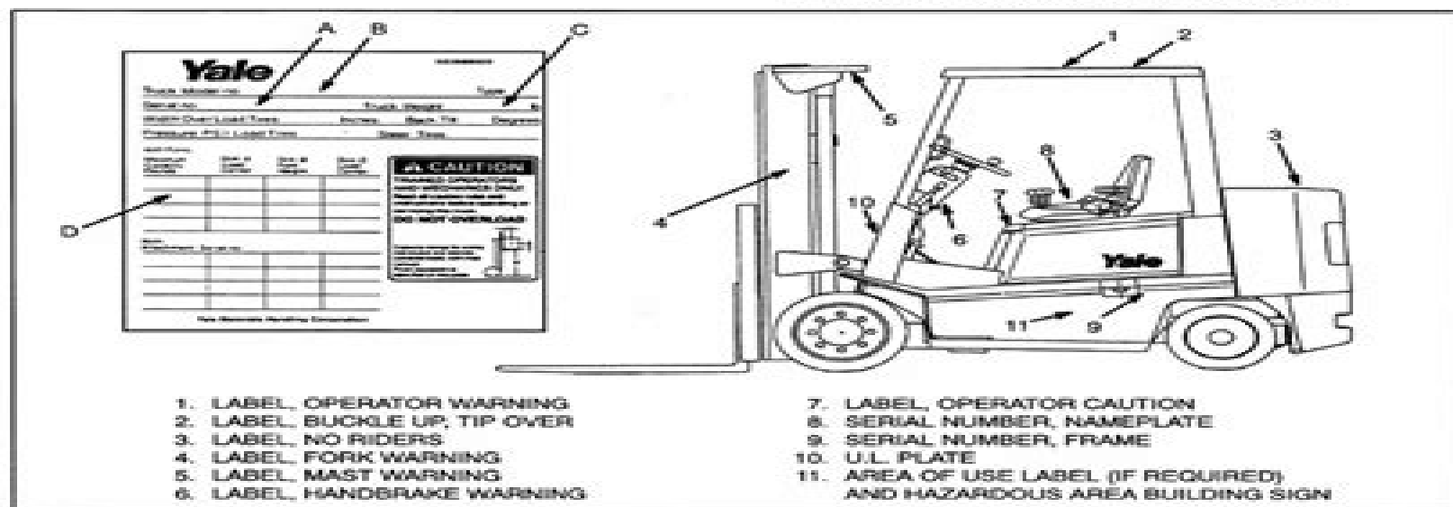
Figure 1-1 - Serial Number Nameplate and Warning Label Locations
