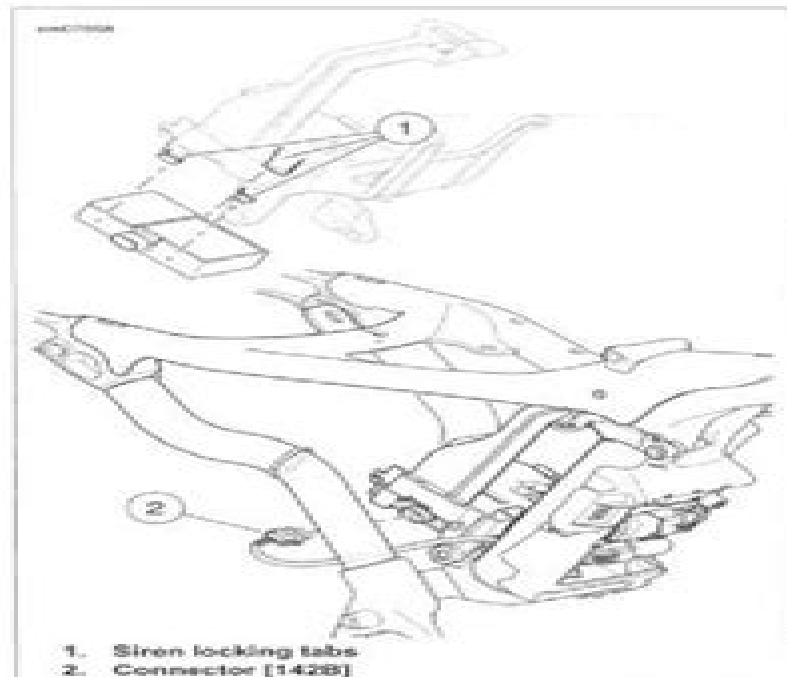
Figure 6-13. Smart Siren
