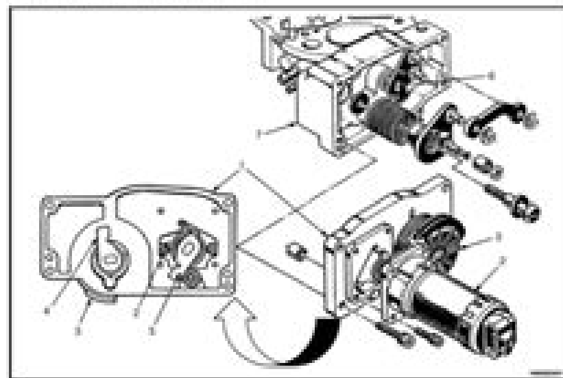
Figure 65. Governor Motor and Throttle Drive Assembly
