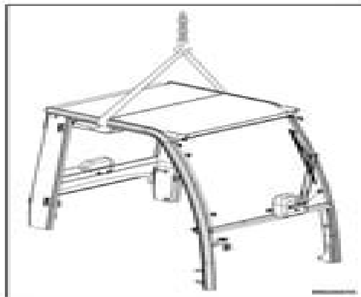
Figure 15. Lift Strap Connection
