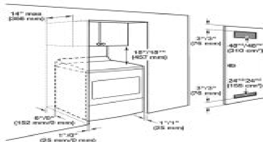
Recommended/Minimum spacing
