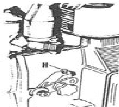
Fig. KR1-2—High speed on variable speed engines is adjusted by turning adjusting screw (H).
