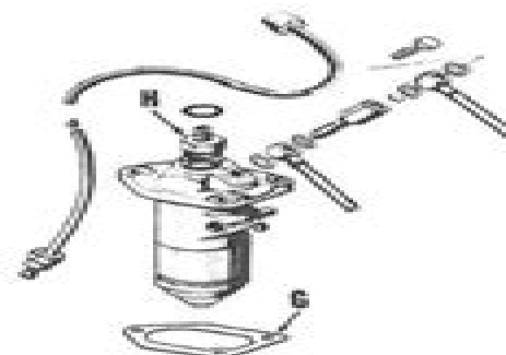
Fig. KR1-3—Injection timing is adjusted by varying thickness of shim gasket (G). Refer to text for timing procedure.
