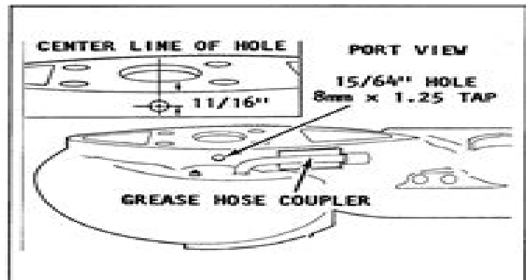
Fig. 40 On models not equipped with a flushing plug, a hole should be drilled and tapped to receive a plug as illustrated.
