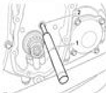
1. Camshaft Timing Pin (T488040) 2. Timing hole in position
