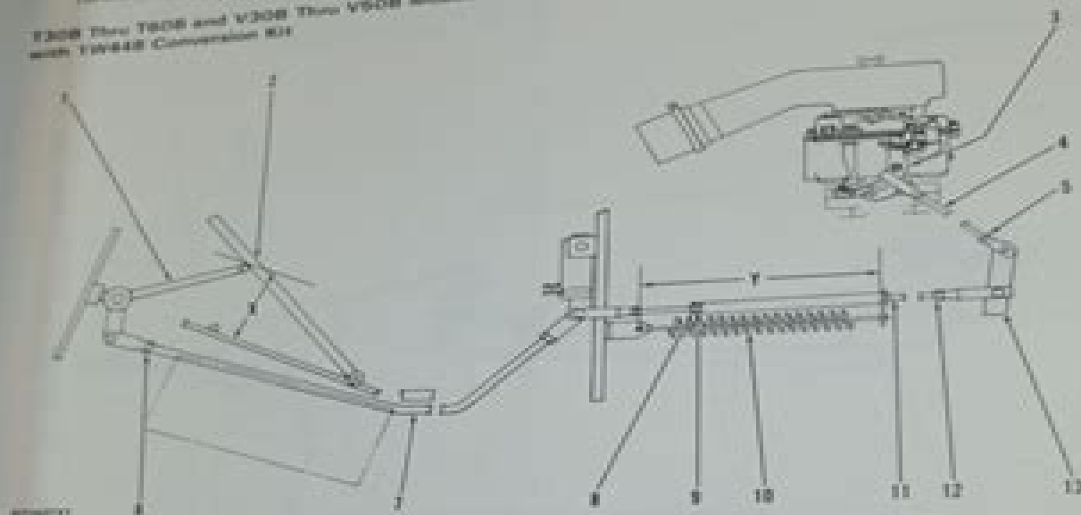
T308 THRU T608 AND V308 THRU V508 CARBURETOR — GOVERNOR LINKAGE (WITH TW448 CONVERSION KIT)
