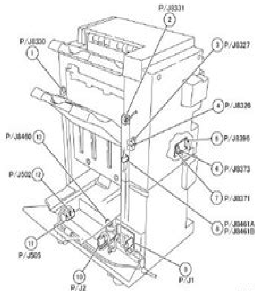
Figure 49 Finisher PWDLVPS (J6u71052)
