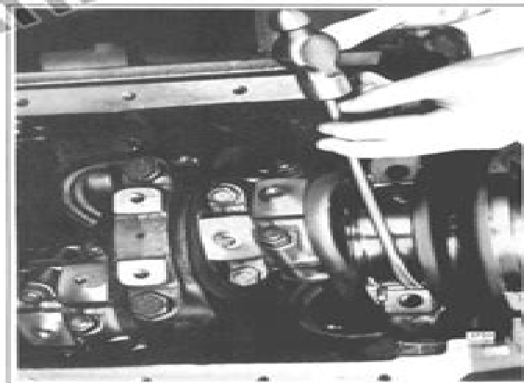
Fig. 5 – Removing Upper Rear Main Bearing Shell
