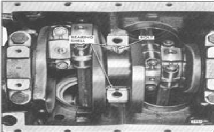
Fig. 4 – Removing Upper Main Bearing Shell (Except Rear Main)
