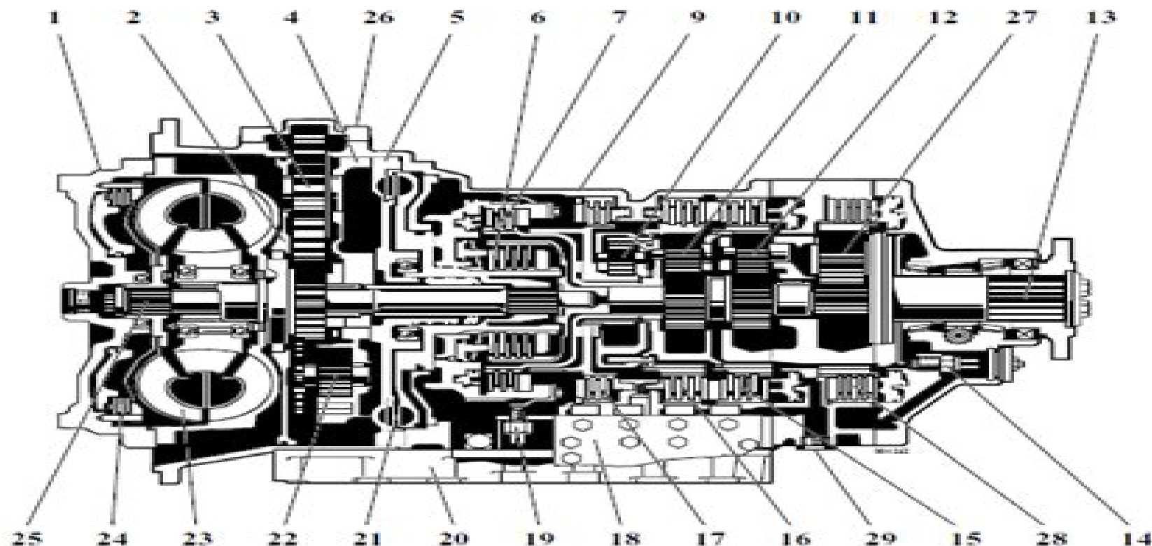
ZF-Ecomat transmission, 5-speed, "long" version
